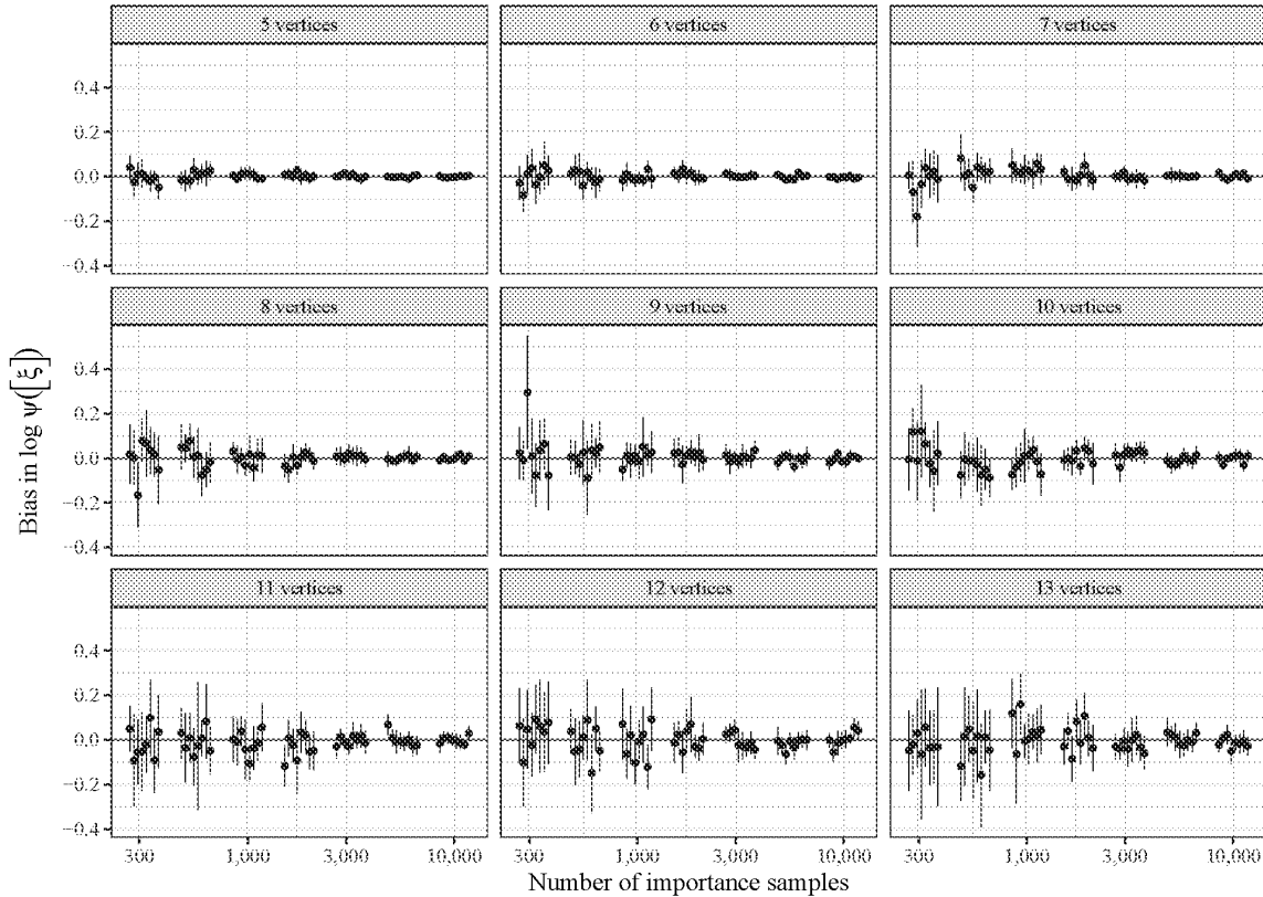
Figure C.4: Bias in importance sampling estimates of \log \psi(\xi) by the number of importance samples and the number of vertices in the district-level graph. District-level graphs were selected as random subsets of the graph shown in C.3. Eight replicate experiments were performed for each importance sample size and graph size. The vertical bars for each point span two standard errors in either direction. Standard errors were calculated with the delta method.
